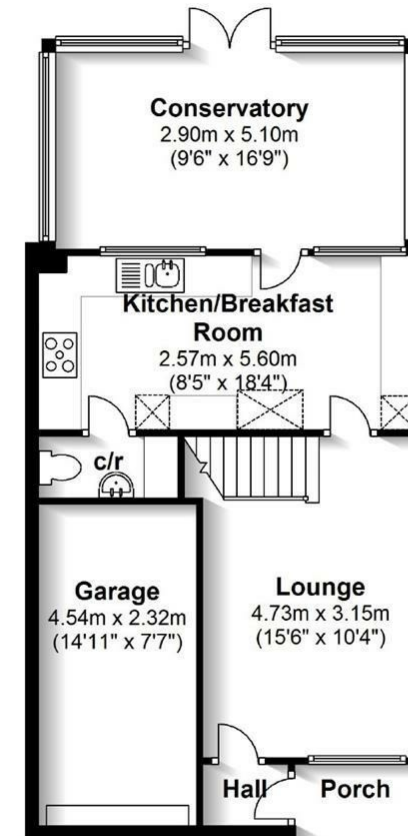
Ground Floor Approx. 62.2 sq. metres (670.0 sq. feet)
