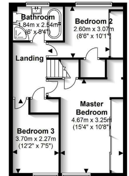
First Floor Approx. 47.1 sq. metres (506.7 sq. feet)
